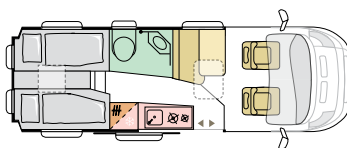
640 SLB | TWIN 60Y L Betten
